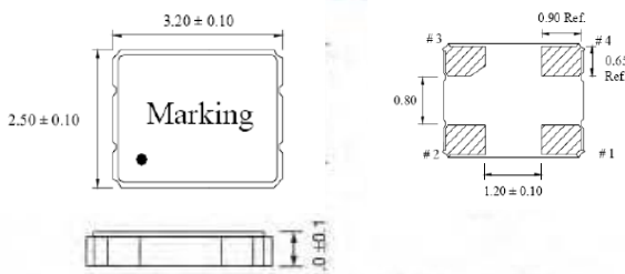
Figure 1) ISO-5X3.2 Top, Side and Bottom views
